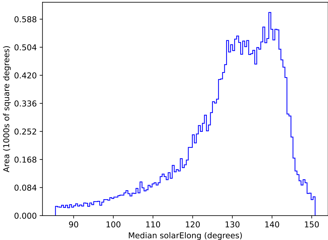
ddf_loaded_half_fl8_v3.4_10yrs All sky all bands: Median solarElong
