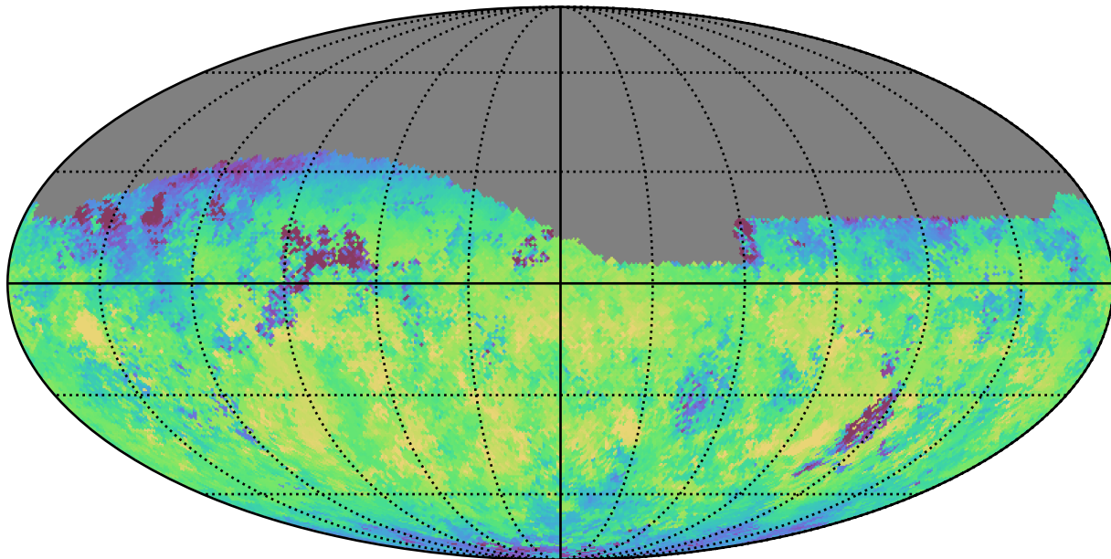
ddf_loaded_half_fl8_v3.4_10yrs Yr 1 z band: Median skyBrightness
