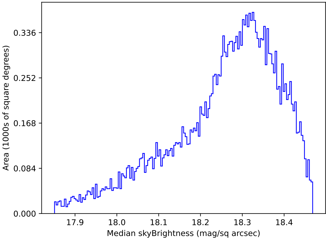
ddf_loaded_half_fl8_v3.4_10yrs Yr 1 y band: Median skyBrightness
