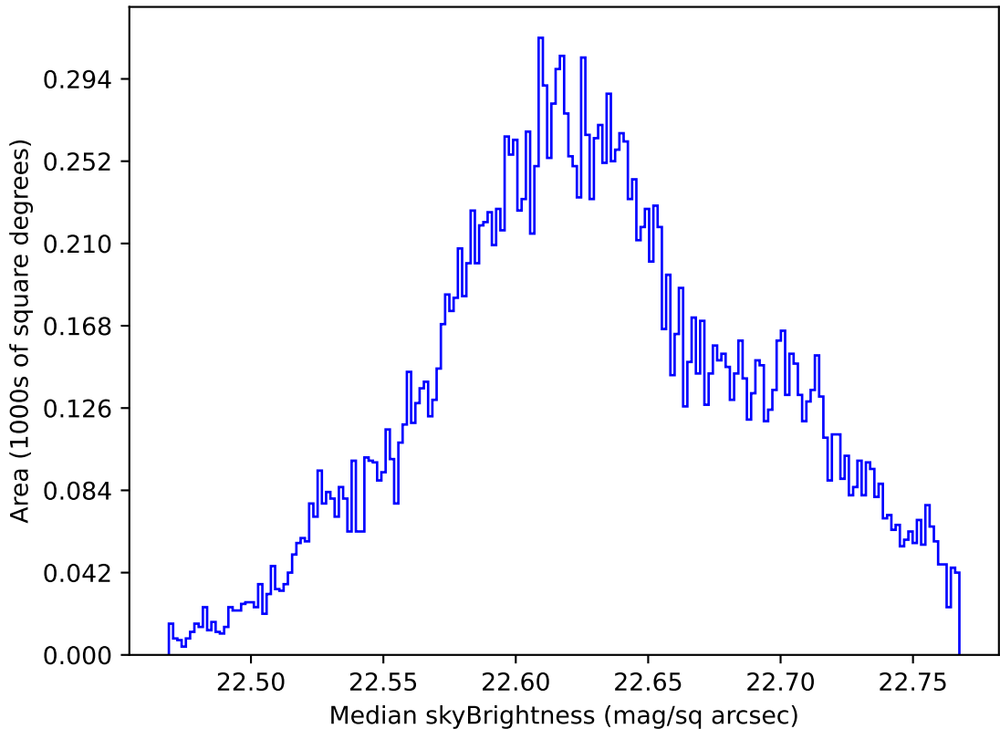
ddf_loaded_half_fl8_v3.4_10yrs Yr 1 u band: Median skyBrightness
