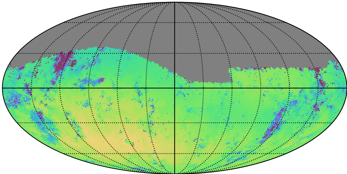
ddf_loaded_half_fl8_v3.4_10yrs Yr 1 g band: Median skyBrightness
