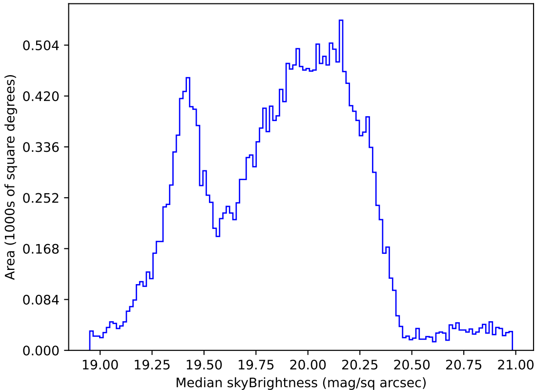
ddf_loaded_half_fl8_v3.4_10yrs Yr 1 all bands: Median skyBrightness
