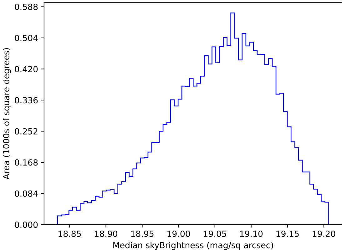
ddf_loaded_half_fl8_v3.4_10yrs WFD z band: Median skyBrightness
