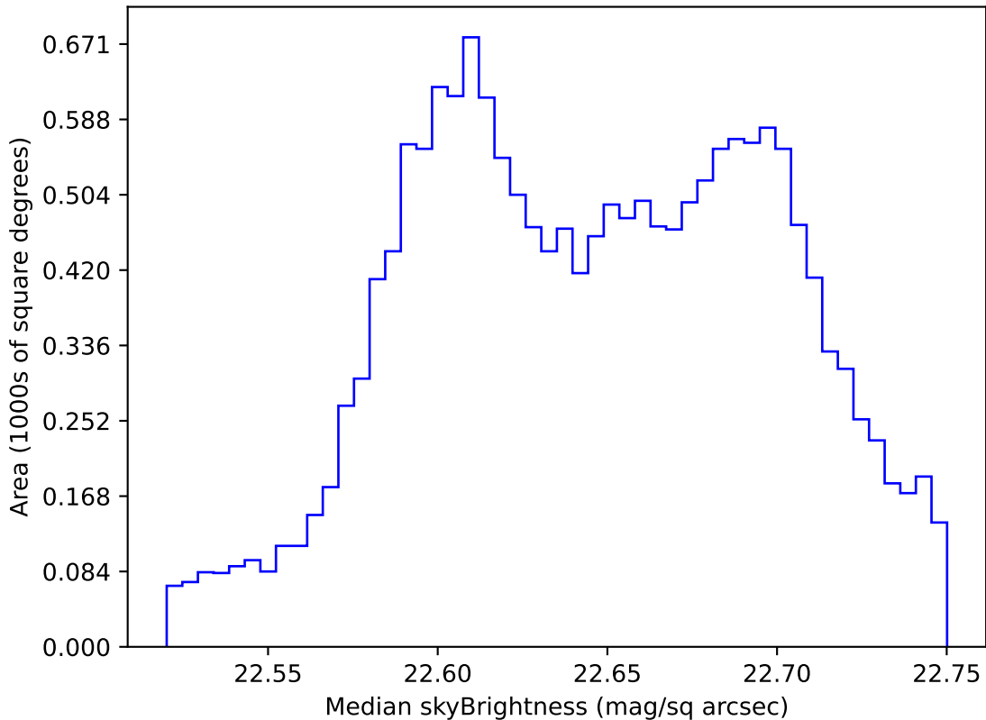
ddf_loaded_half_fl8_v3.4_10yrs WFD u band: Median skyBrightness
