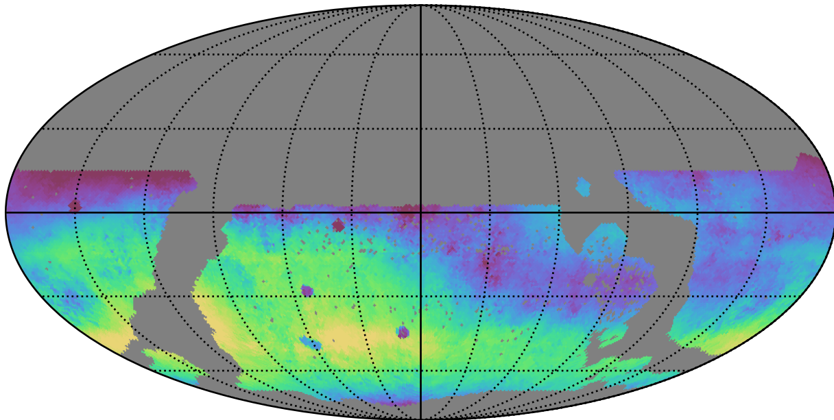
ddf_loaded_half_fl8_v3.4_10yrs WFD r band: Median skyBrightness
