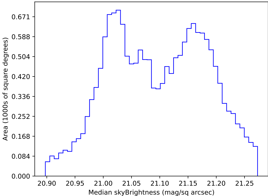
ddf_loaded_half_fl8_v3.4_10yrs WFD r band: Median skyBrightness
