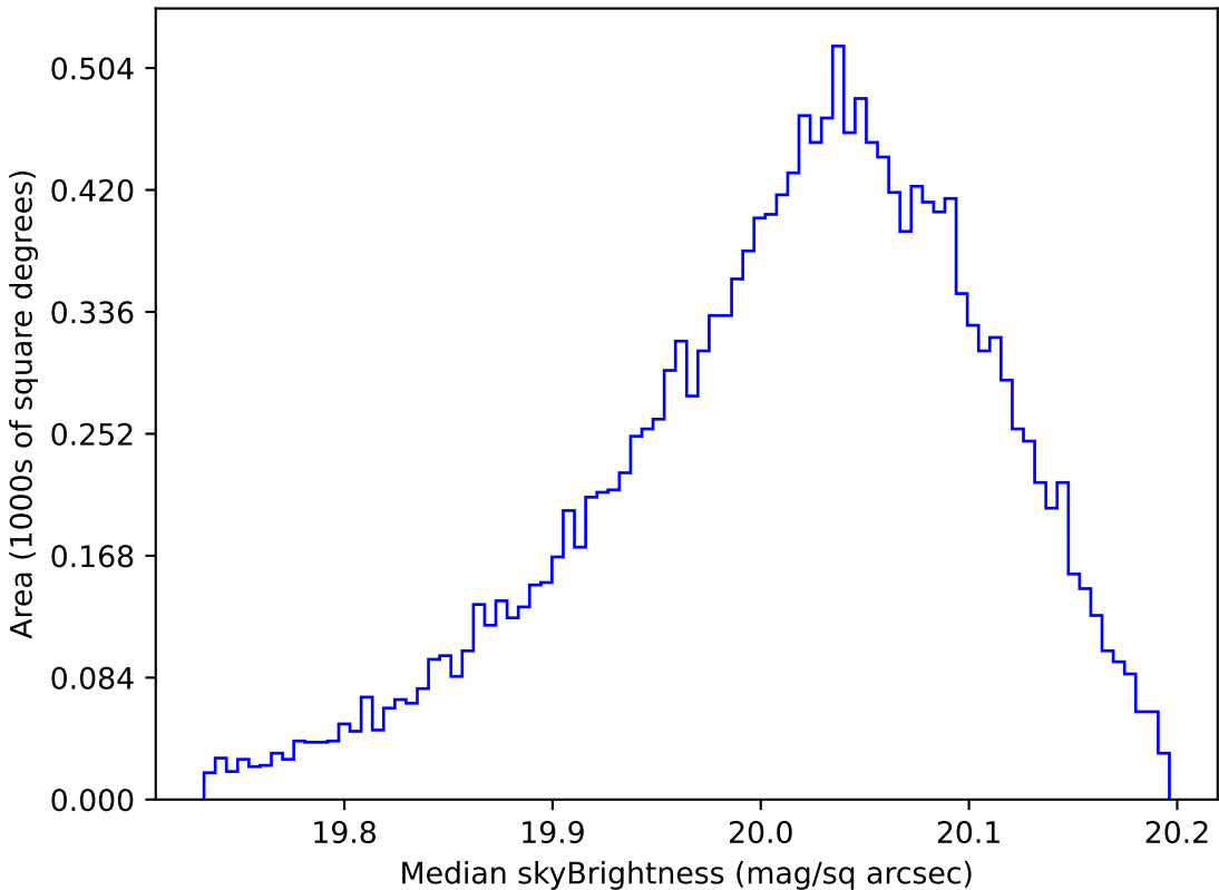
ddf_loaded_half_fl8_v3.4_10yrs WFD i band: Median skyBrightness
