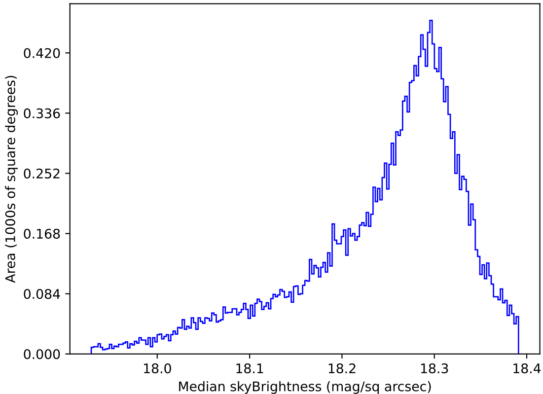
ddf_loaded_half_fl8_v3.4_10yrs All sky y band: Median skyBrightness
