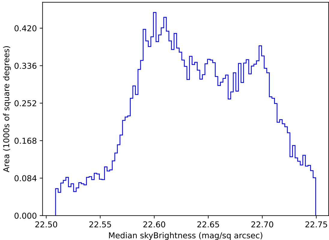
ddf_loaded_half_fl8_v3.4_10yrs All sky u band: Median skyBrightness
