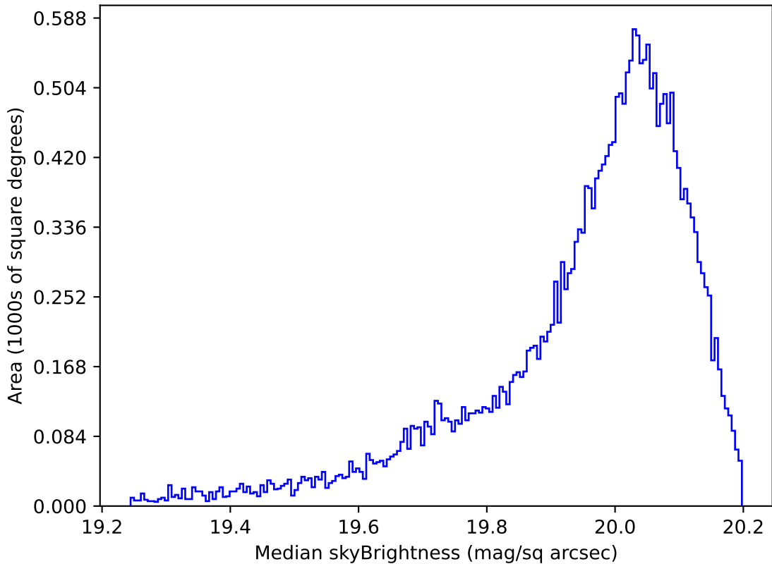
ddf_loaded_half_fl8_v3.4_10yrs All sky i band: Median skyBrightness
