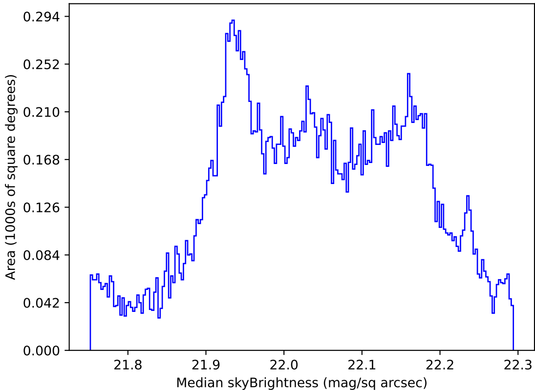
ddf_loaded_half_fl8_v3.4_10yrs All sky g band: Median skyBrightness
