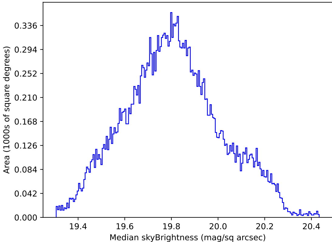
ddf_loaded_half_fl8_v3.4_10yrs All sky all bands: Median skyBrightness
