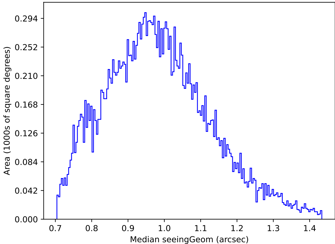
ddf_loaded_half_fl8_v3.4_10yrs Yr 1 u band: Median seeingGeom
