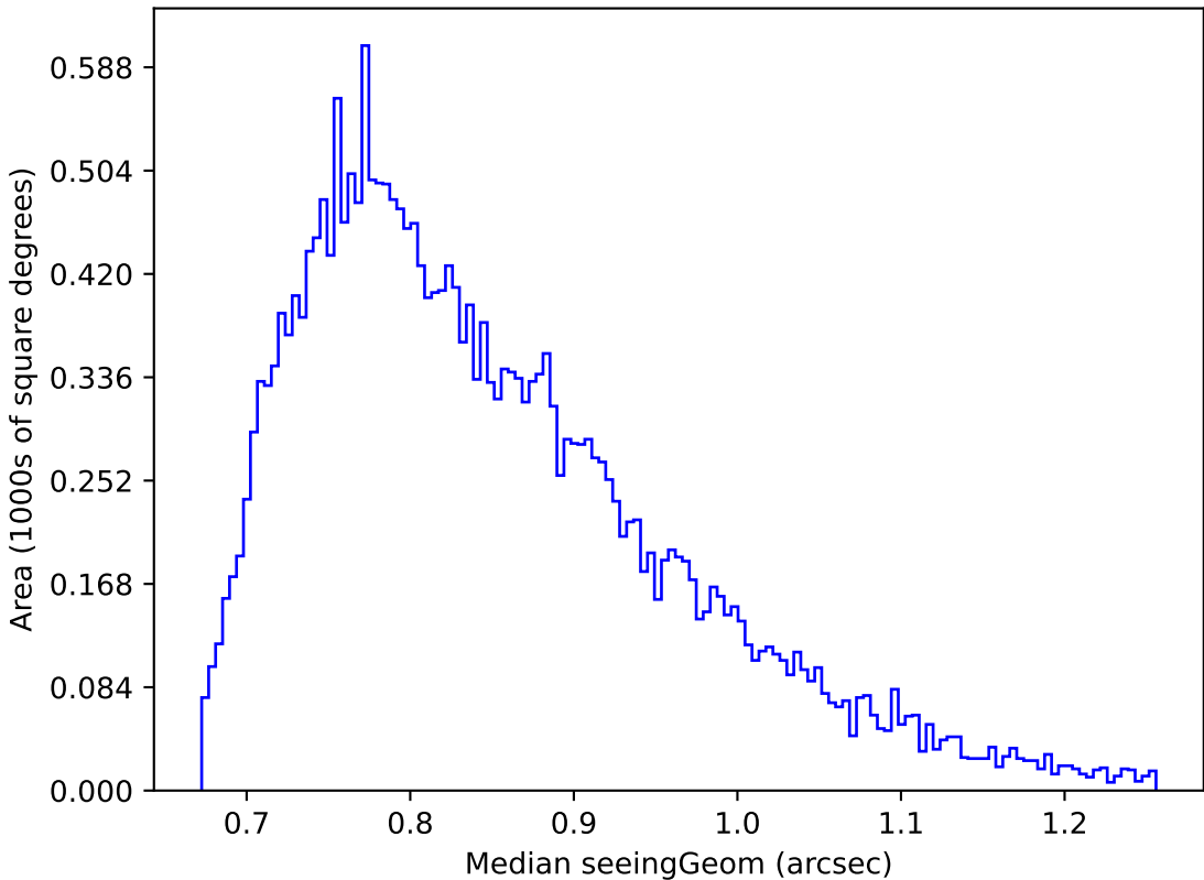
ddf_loaded_half_fl8_v3.4_10yrs Yr 1 r band: Median seeingGeom
