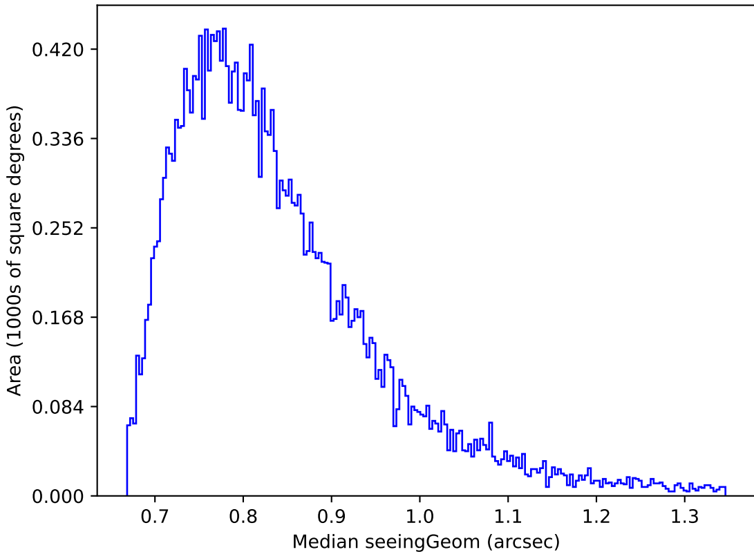
ddf_loaded_half_fl8_v3.4_10yrs Yr 1 i band: Median seeingGeom
