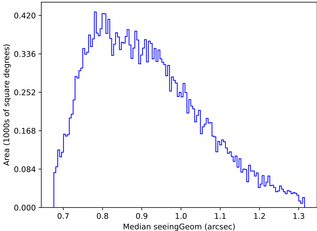
ddf_loaded_half_fl8_v3.4_10yrs Yr 1 g band: Median seeingGeom
