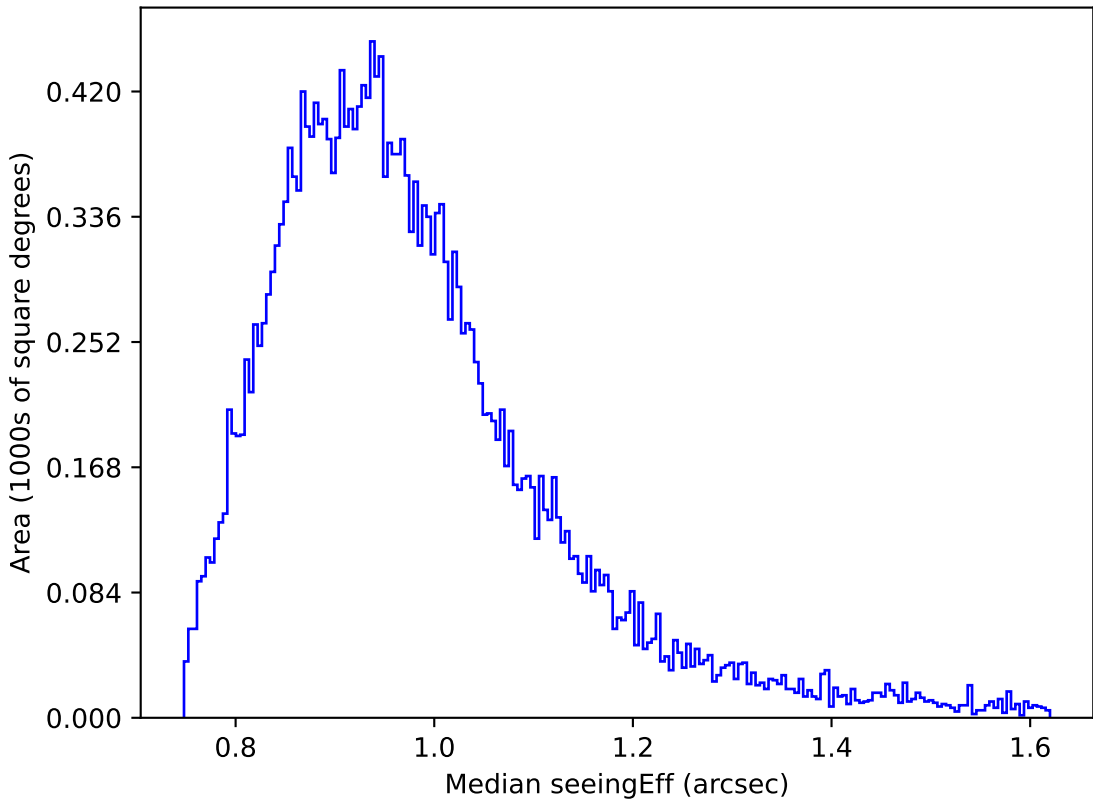
ddf_loaded_half_fl8_v3.4_10yrs Yr 1 z band: Median seeingEff
