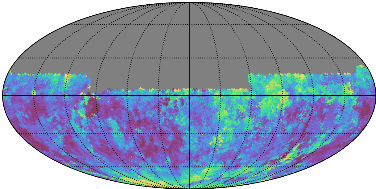
ddf_loaded_half_fl8_v3.4_10yrs Yr 1 y band: Median seeingEff
