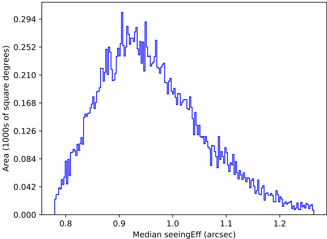
ddf_loaded_half_fl8_v3.4_10yrs Yr 1 y band: Median seeingEff
