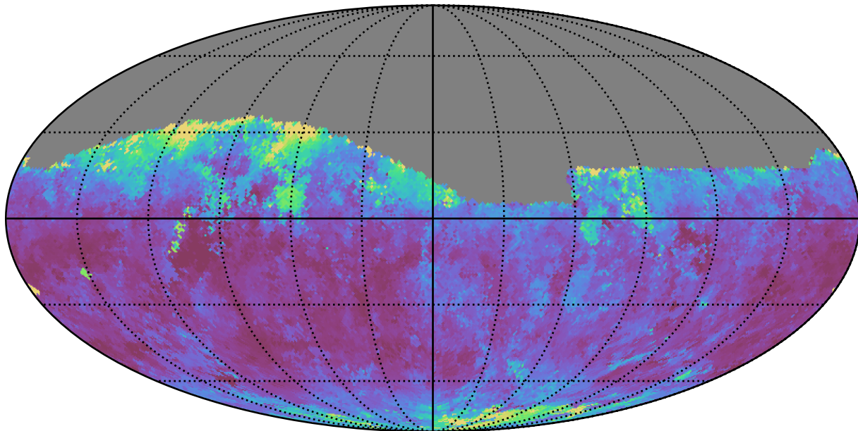
ddf_loaded_half_fl8_v3.4_10yrs Yr 1 i band: Median seeingEff
