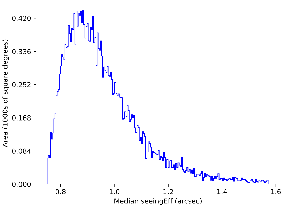
ddf_loaded_half_f18_v3.4_10yrs Yr 1 i band: Median seeingEff
