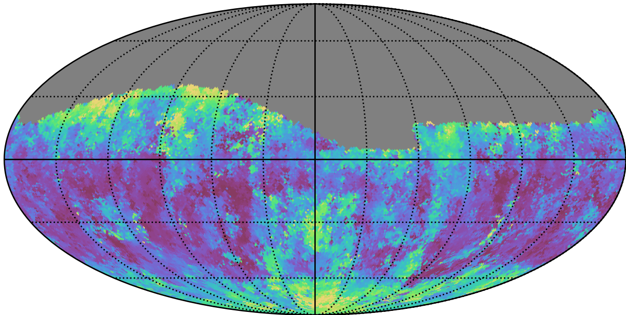
ddf_loaded_half_fl8_v3.4_10yrs Yr 1 g band: Median seeingEff
