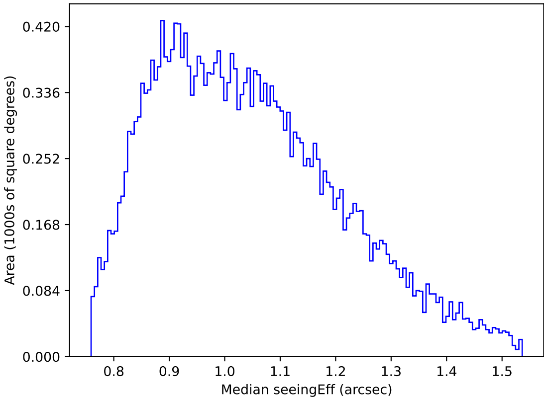
ddf_loaded_half_fl8_v3.4_10yrs Yr 1 g band: Median seeingEff
