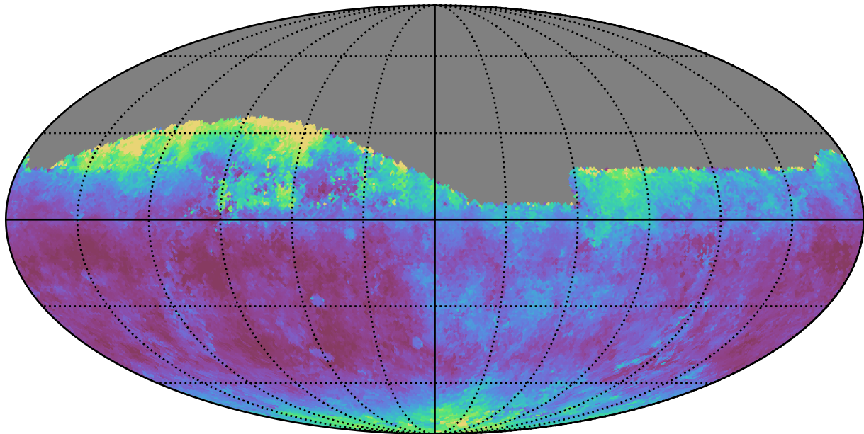
ddf_loaded_half_fl8_v3.4_10yrs Yr 1 all bands: Median seeingEff
