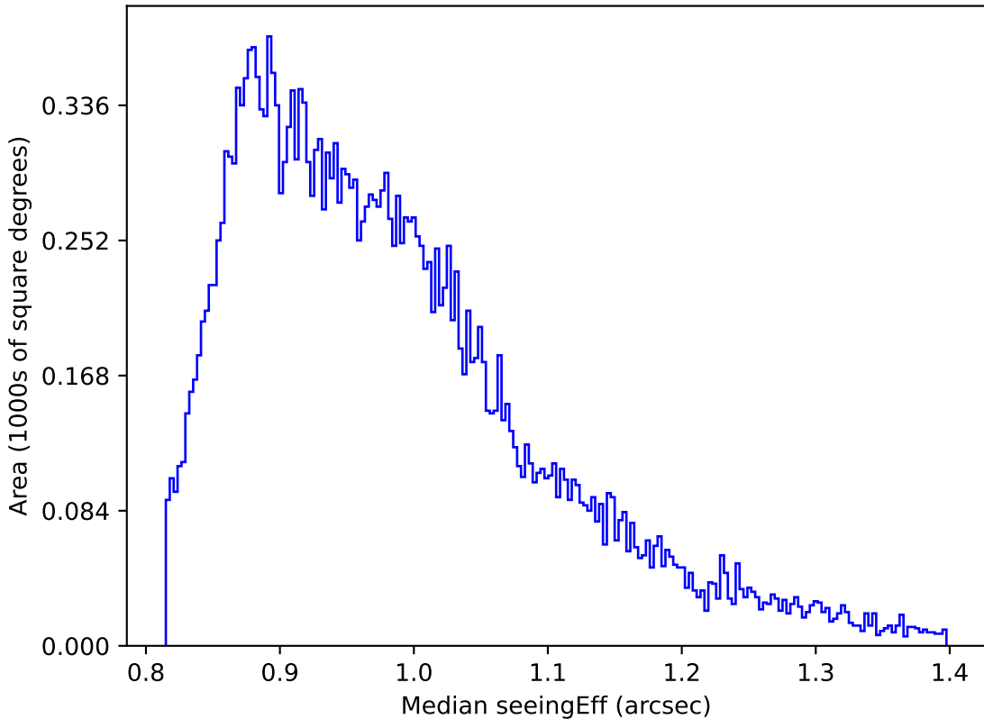
ddf_loaded_half_fl8_v3.4_10yrs Yr 1 all bands: Median seeingEff
