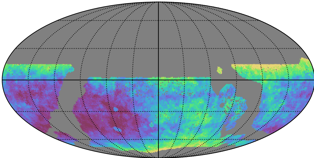
ddf_loaded_half_fl8_v3.4_10yrs WFD z band: Median seeingEff
