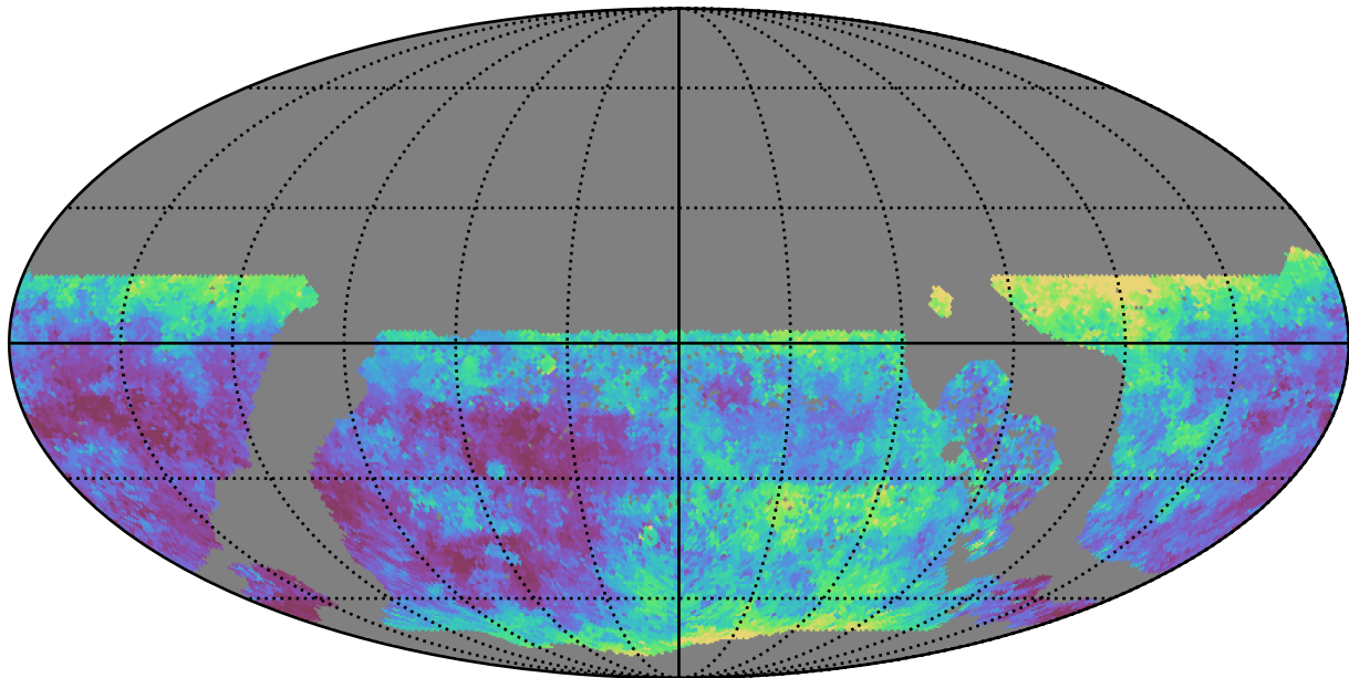
ddf_loaded_half_fl8_v3.4_10yrs WFD u band: Median seeingEff
