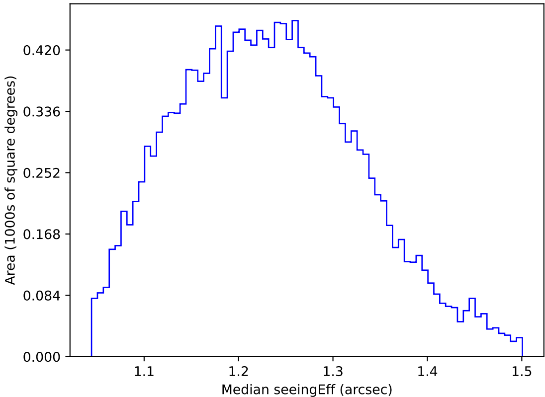
ddf_loaded_half_fl8_v3.4_10yrs WFD u band: Median seeingEff
