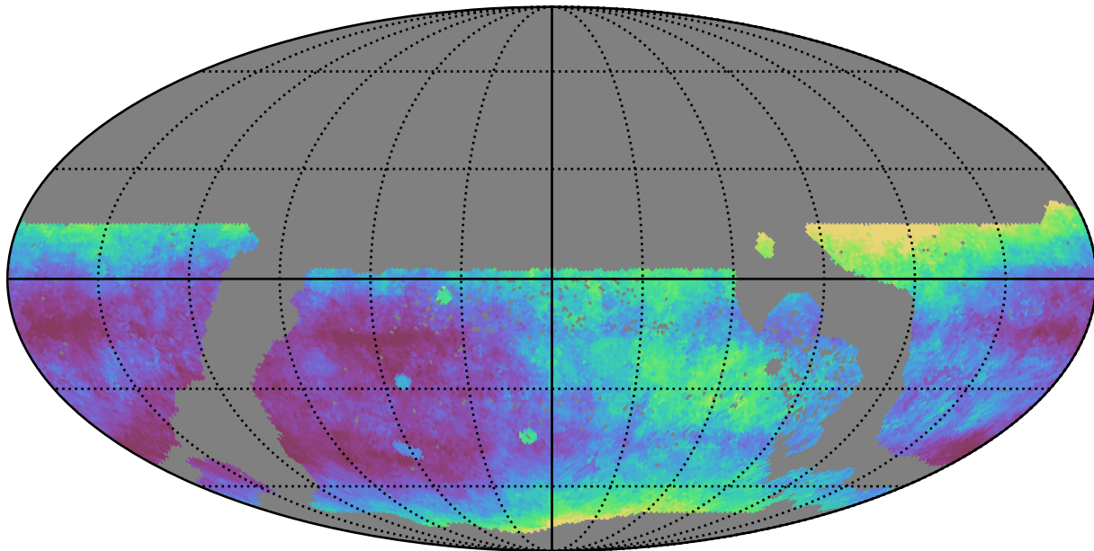
ddf_loaded_half_fl8_v3.4_10yrs WFD r band: Median seeingEff
