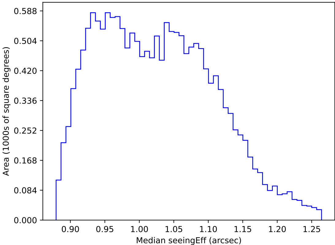
ddf_loaded_half_fl8_v3.4_10yrs WFD r band: Median seeingEff
