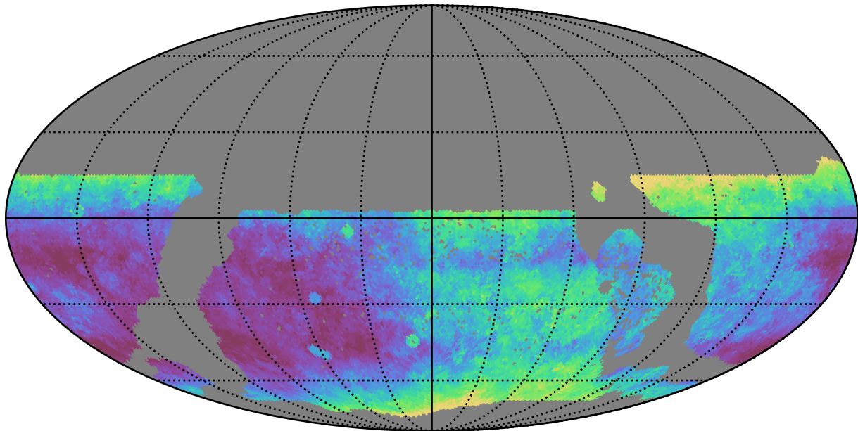
ddf_loaded_half_fl8_v3.4_10yrs WFD i band: Median seeingEff
