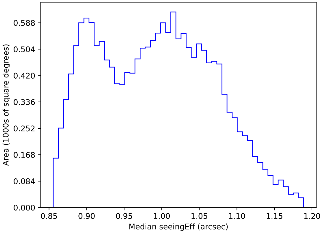
ddf_loaded_half_fl8_v3.4_10yrs WFD i band: Median seeingEff
