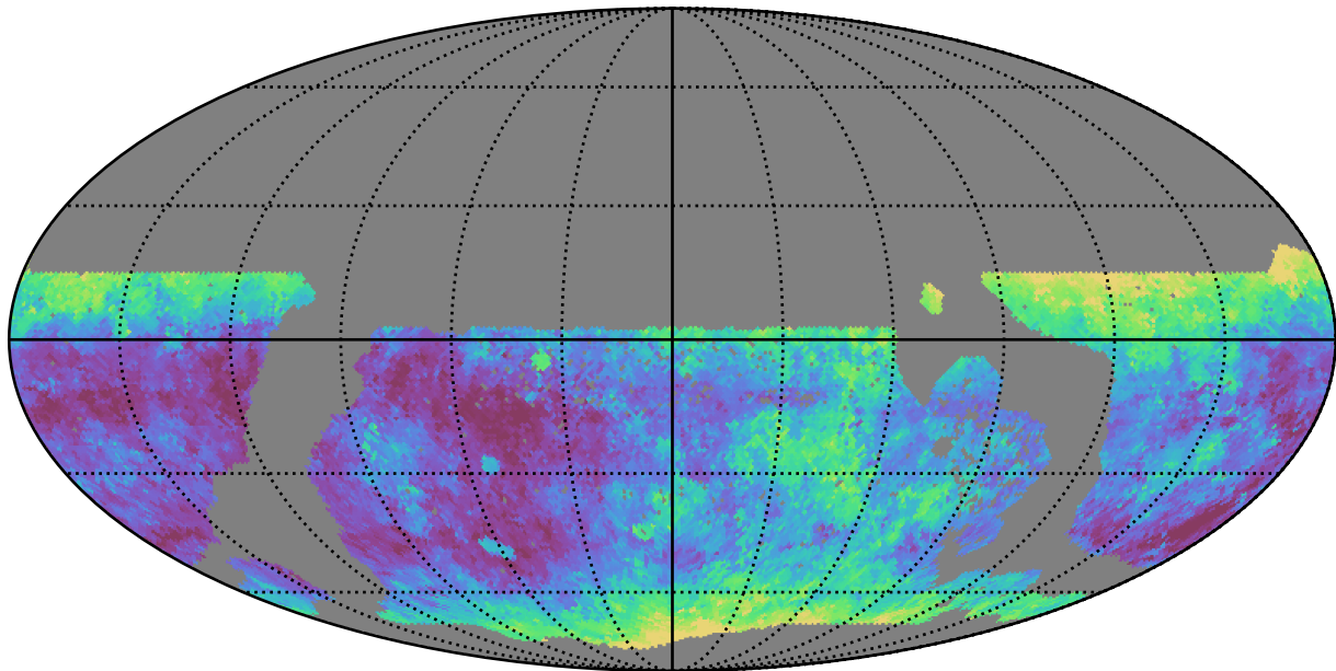
ddf_loaded_half_fl8_v3.4_10yrs WFD g band: Median seeingEff
