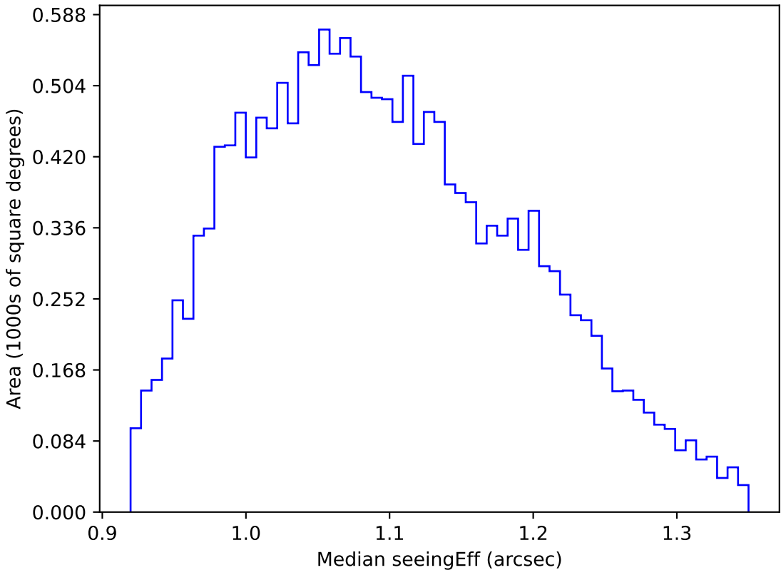
ddf_loaded_half_fl8_v3.4_10yrs WFD g band: Median seeingEff
