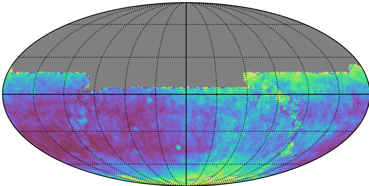
ddf_loaded_half_fl8_v3.4_10yrs All sky y band: Median seeingEff
