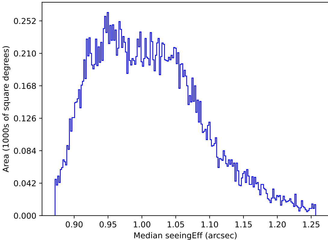
ddf_loaded_half_fl8_v3.4_10yrs All sky y band: Median seeingEff
