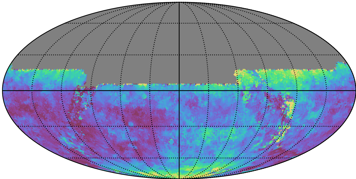
ddf_loaded_half_fl8_v3.4_10yrs All sky u band: Median seeingEff
