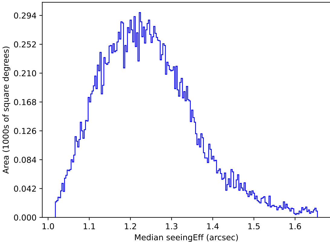
ddf_loaded_half_fl8_v3.4_10yrs All sky u band: Median seeingEff
