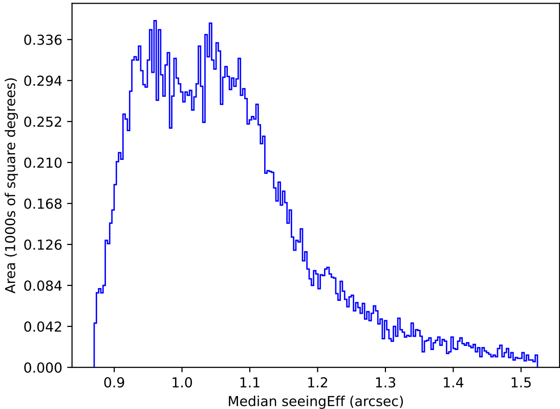
ddf_loaded_half_fl8_v3.4_10yrs All sky r band: Median seeingEff
