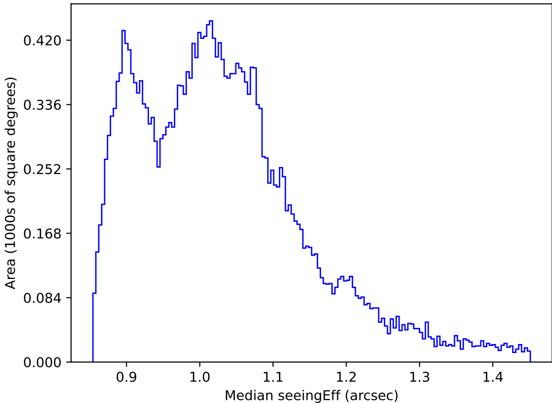
ddf_loaded_half_fl8_v3.4_10yrs All sky i band: Median seeingEff
