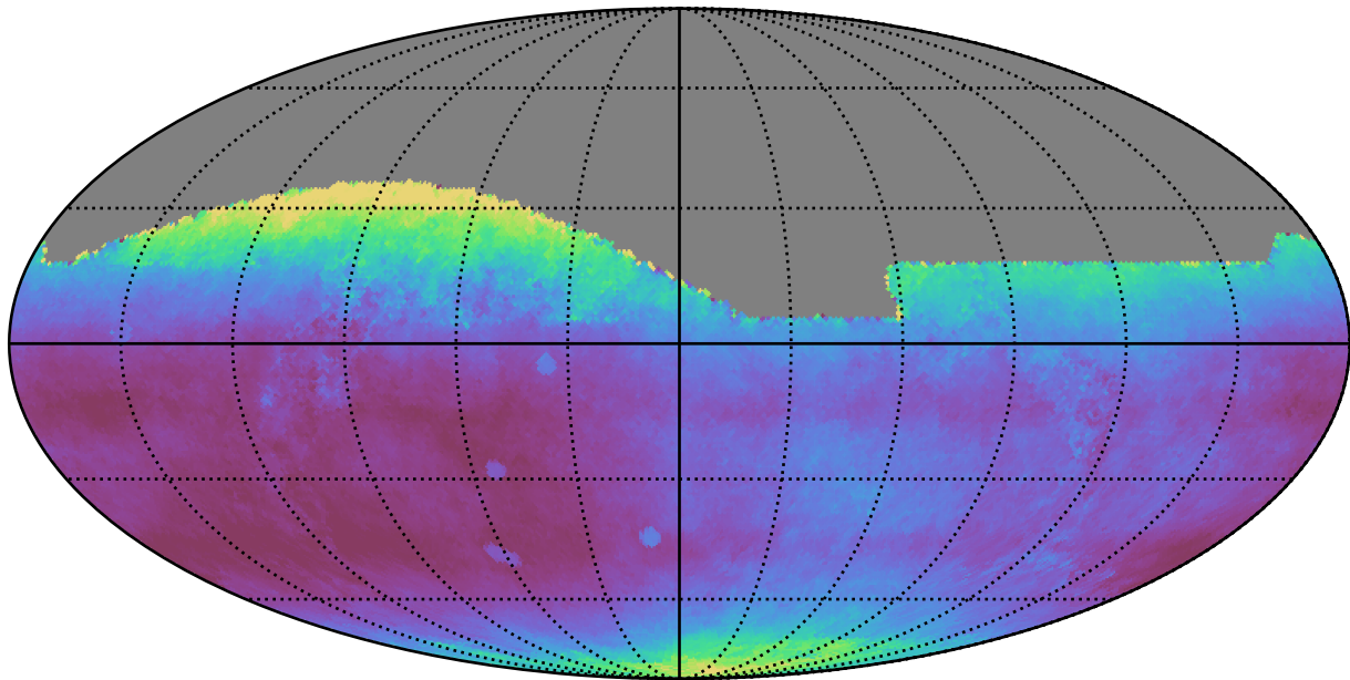
ddf_loaded_half_fl8_v3.4_10yrs All sky all bands: Median seeingEff
