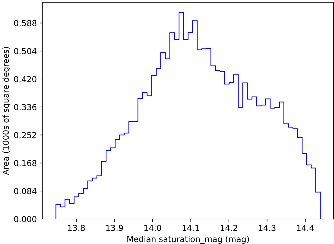
ddf_loaded_half_fl8_v3.4_10yrs WFD z band: Median saturation_mag
