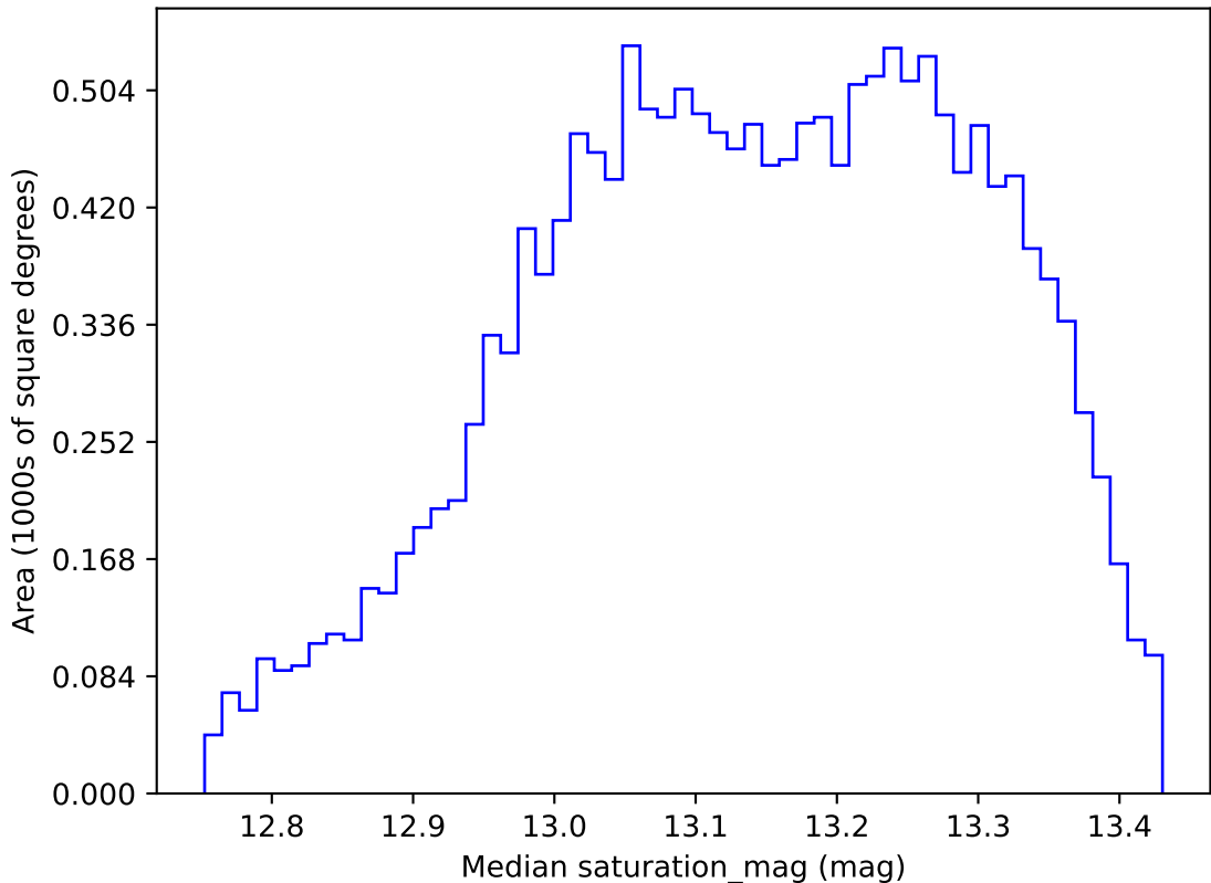
ddf_loaded_half_fl8_v3.4_10yrs WFD y band: Median saturation_mag
