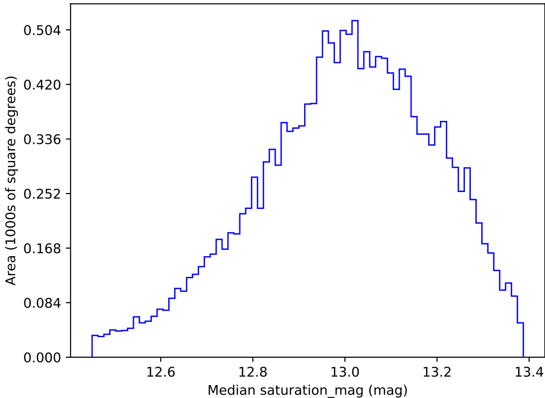
ddf_loaded_half_fl8_v3.4_10yrs WFD u band: Median saturation_mag
