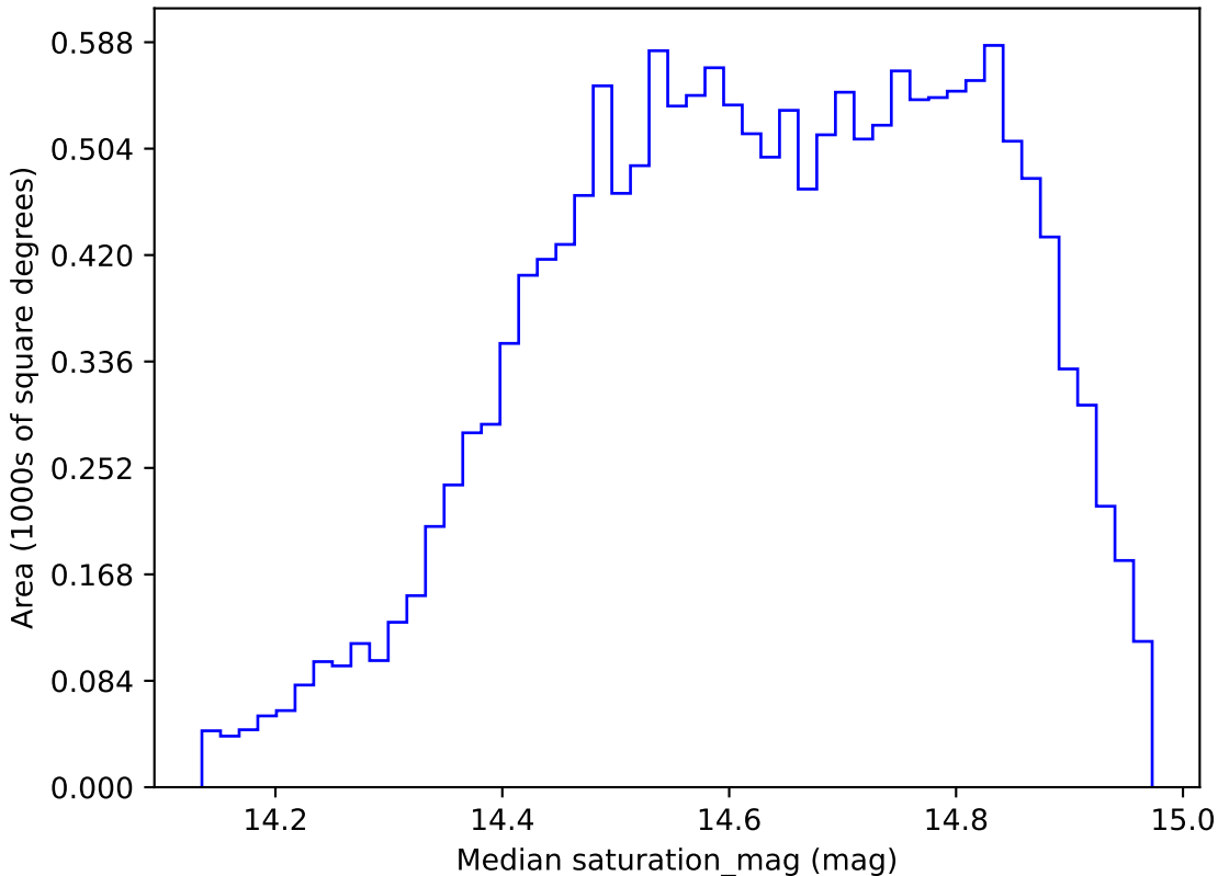
ddf_loaded_half_fl8_v3.4_10yrs WFD r band: Median saturation_mag
