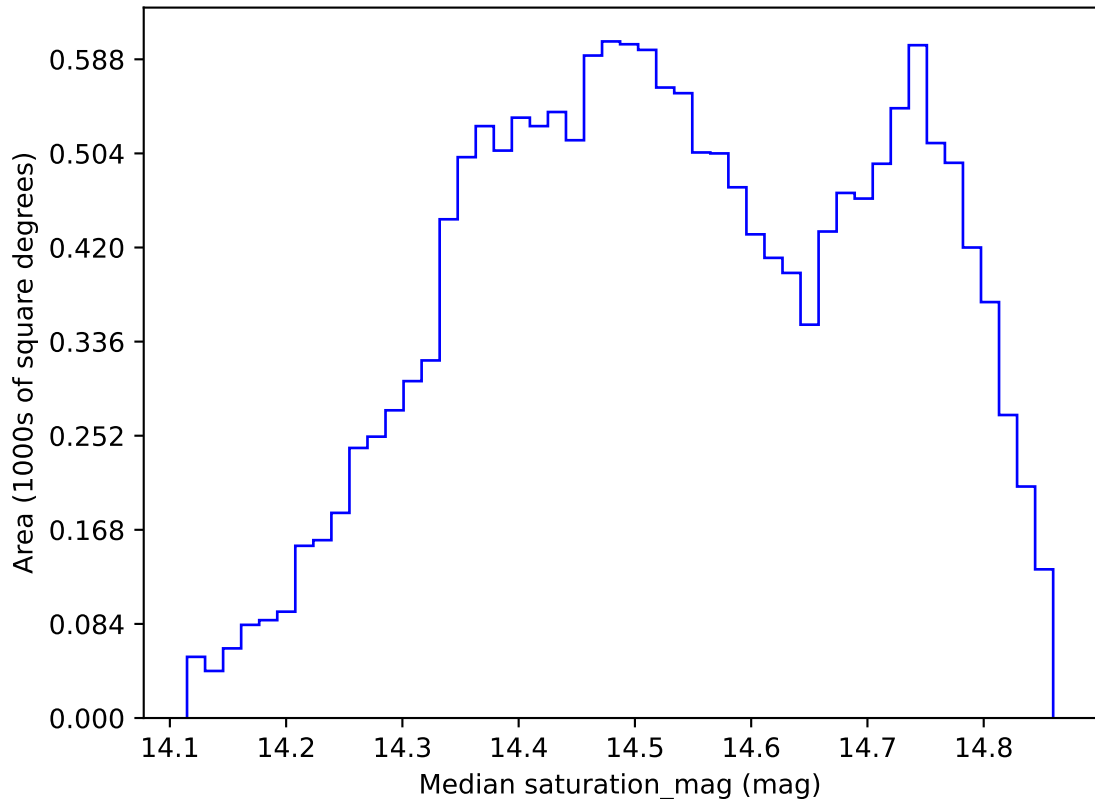
ddf_loaded_half_fl8_v3.4_10yrs WFD i band: Median saturation_mag
